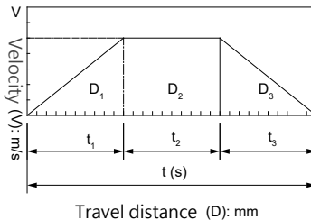
Fig. 6.1.2 Velocity Diagram
